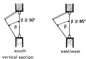
27 Reduction factor z of solar protection devices in association with glazing types
